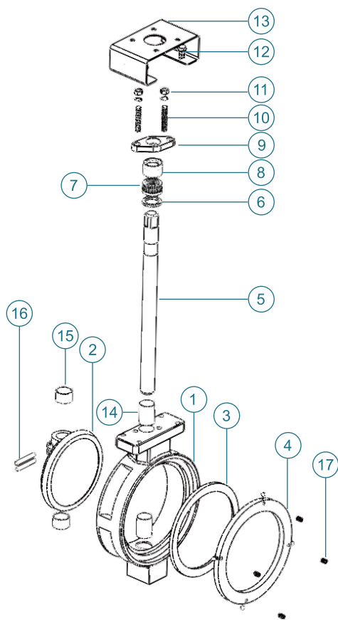
Wafer type
